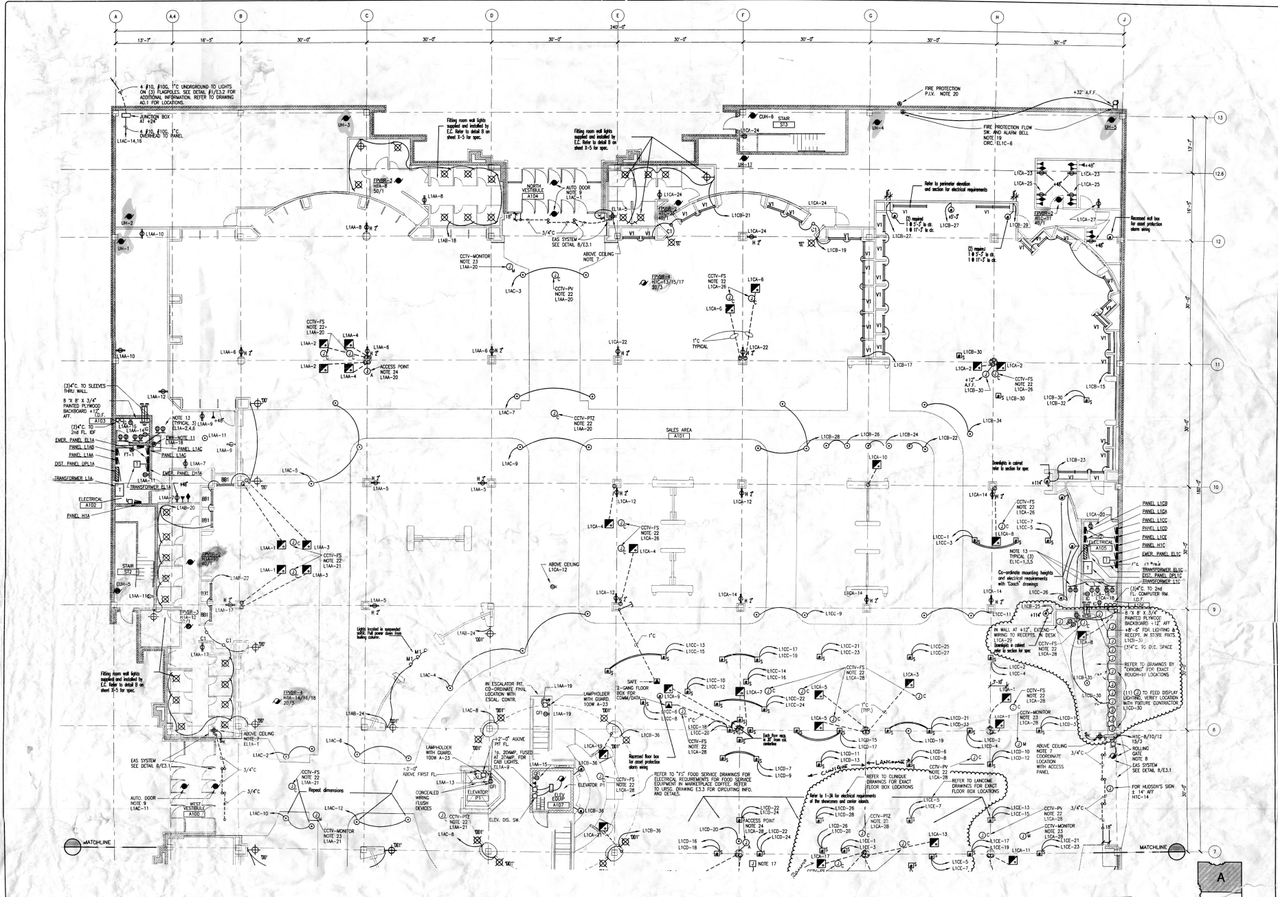
FIRST FLOOR PLAN - AREA "A" F.F.E. = 100'-0"
