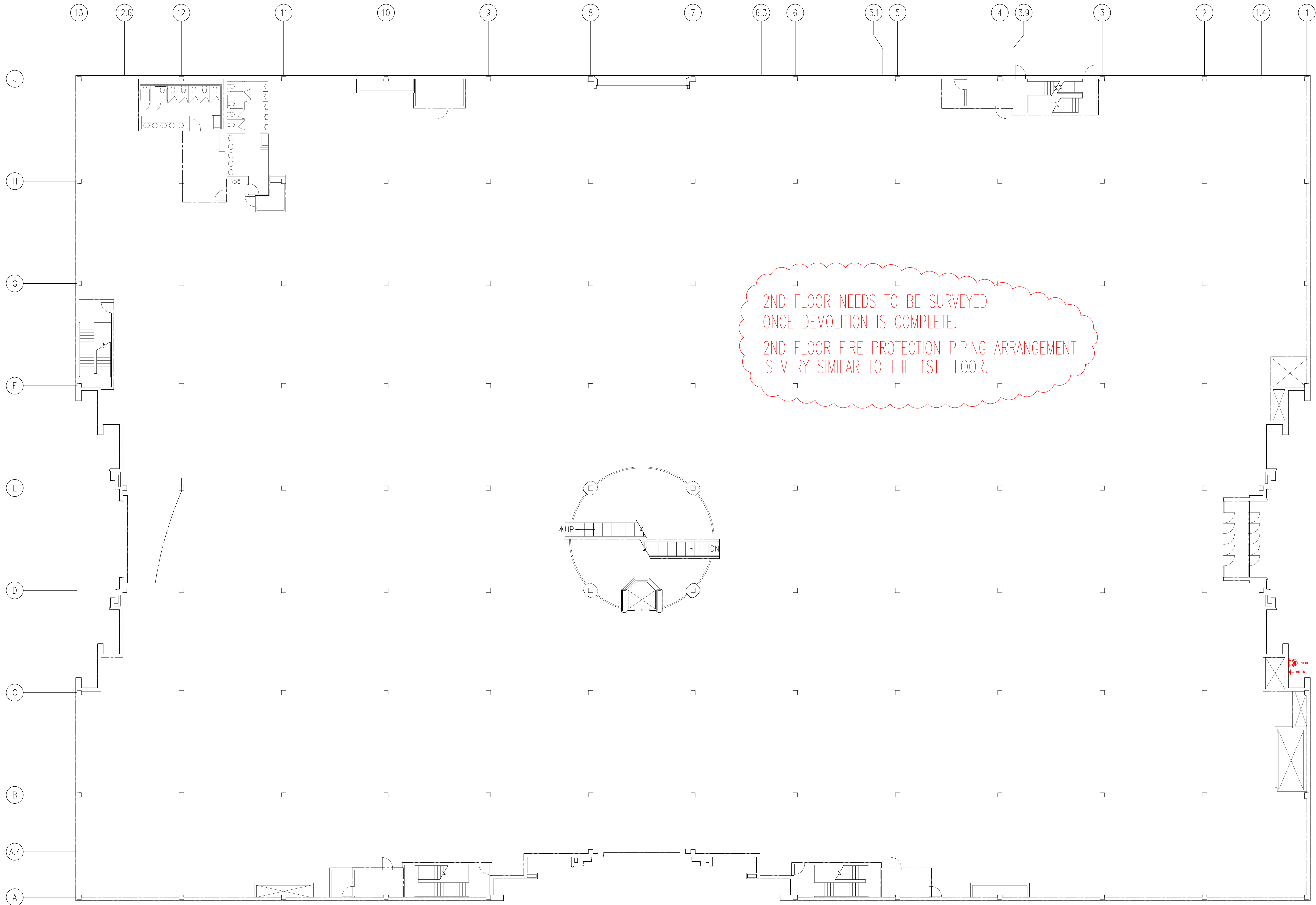
2nd Floor Existing Sprinkler Piping Layout 3/32" = 1'-0"
