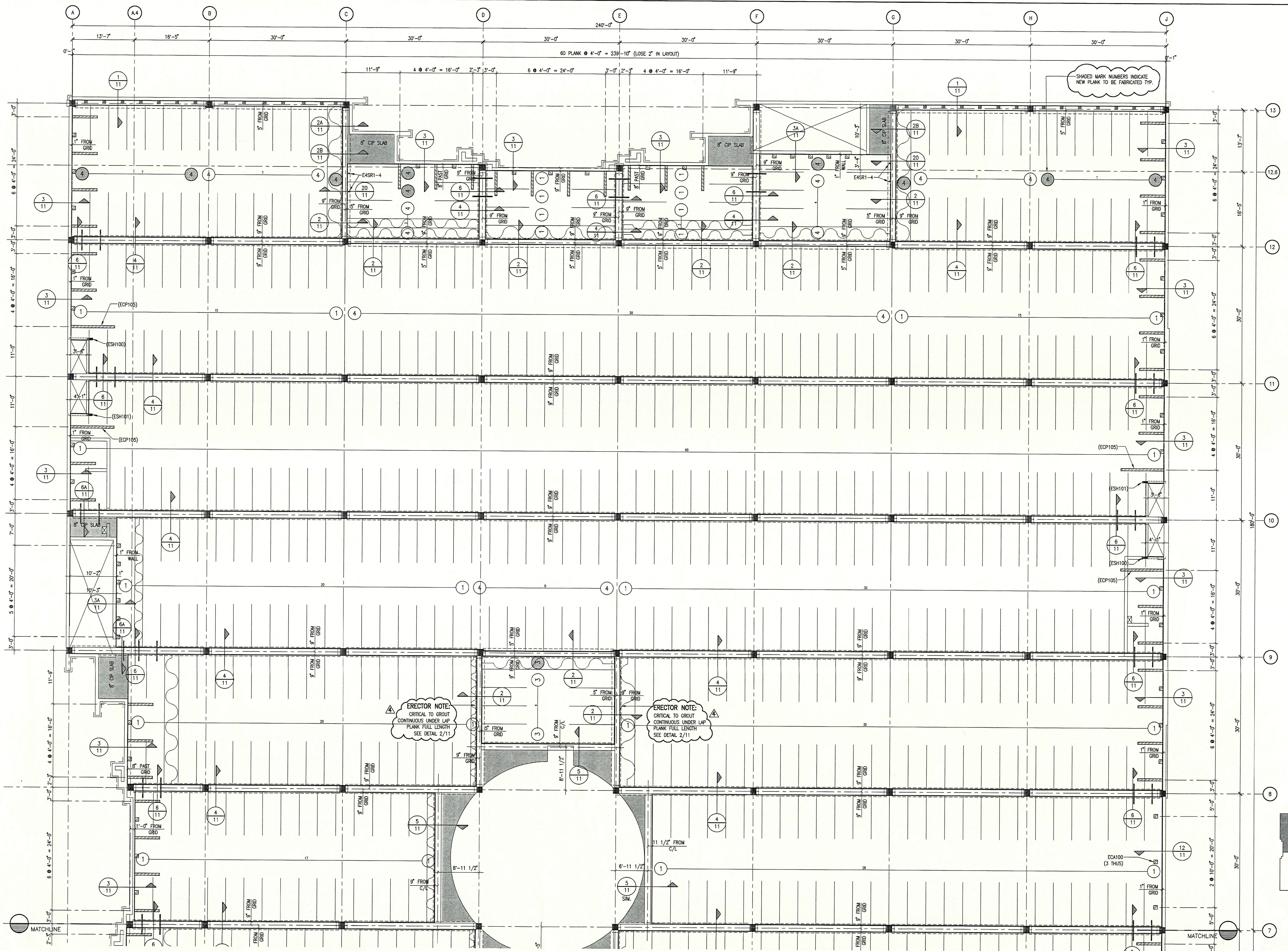
1 12" SPANGRETE LAYOUT - 2nd FLOOR - AREA "A" 5 SCALE: 1/8" = 1'-0"
